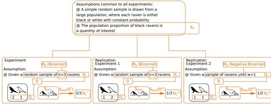
Fig. 1 Elements of three idealized experiments: experiment, replication experiment 1, and an alternative replication experiment 2.
