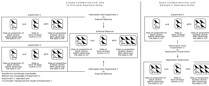
Fig. 2 Closed collaboratorium: Experiment 1 starts with prior view of 1/2 on proportion of black ravens. Observes 2 black ravens and updates their view to 3/4 . Identical view, model, and methods are assumed and the same data values are observed in Experiment 1', but in the absence of an external observer the two results cannot be connected, thus reproducibility is only in principle and evidence does not accumulate in the absence of an external observer privy to both experiments. Open collaboratorium: Experiment 1 starts with prior view of 1/2 on proportion of black ravens. Observes 2 black ravens and updates their view to 3/4 . Experiment 1'—a replication experiment—is informed of the result, model, methods and observes the same data values. Starting with a view of 3/4 they update the proportion of black ravens to 5/6 . Thus, Experiment 1' learns from Experiment 1 in a planned manner. The two results can be connected and thus reproducibility is epistemic .
